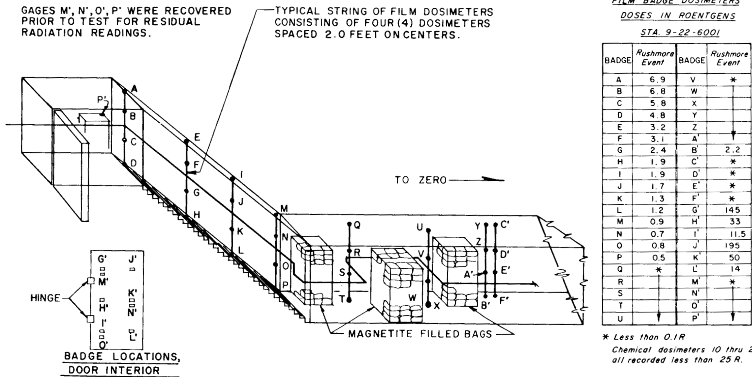
Fig. 10—Station 9-22-6001, dosimeter locations and readings.
